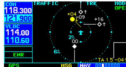
Figure 12-14 Non-Bearing TA Banner
