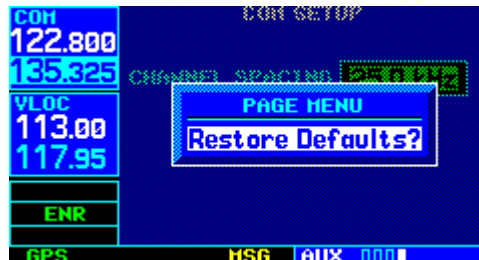
Figure 10-79 COM Setup Page Menu
