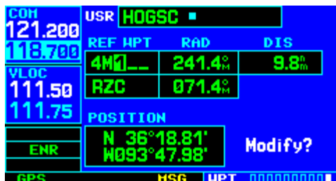
Figure 7-46 Ref Waypoint Field Selected
