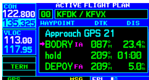
Figure 6-28 Active Flight Plan Page
