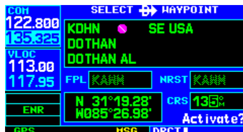
Figure 4-14 Course Field Selected
