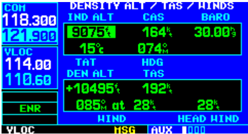
Figure 10-6 Density Alt/TAS/Winds Page
