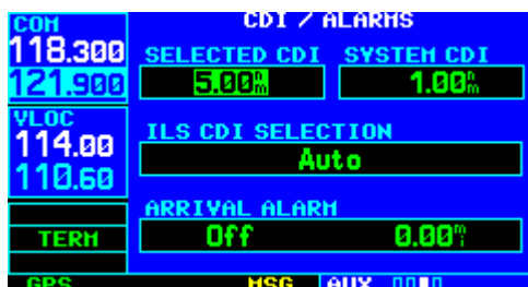
Figure 10-59 Selected CDI Field Highlighted
