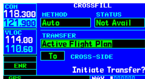
Figure 10-24 Transfer Field Highlighted
