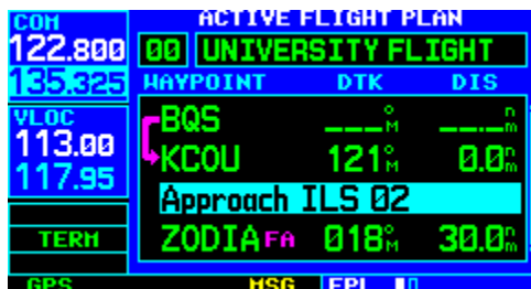
Figure 5-33 Highlight Item To Be Deleted
