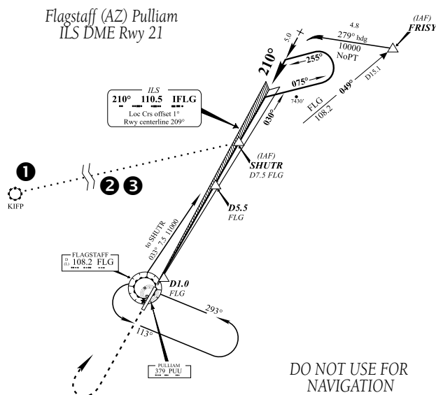
Figure 6-73 ILS Approach, Flagstaff
