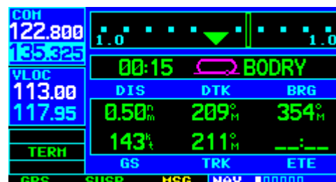
Figure 6-31 Default NAV Page
