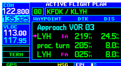
Figure 6-14 Active Flight Plan Page
