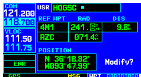
Figure 7-47 Radial Field Selected
