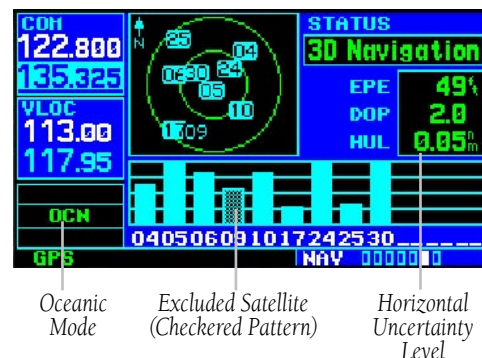
Figure 13-1 Satellite Status Page
