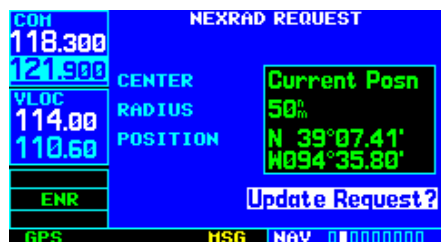
Figure 12-21 NEXRAD Request Page (GDL 69)
