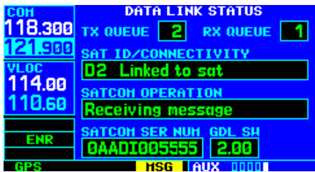
Figure 12-36 Data Link Status Page
