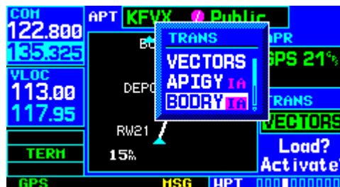
Figure 6-27 TRANS 'Transitions' Window
