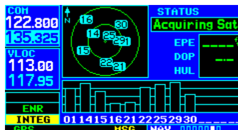
Figure 3-48 Hollow Signal Strength Bars
