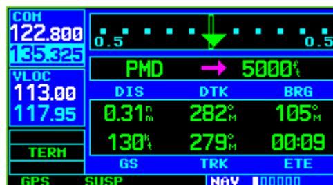
Figure 6-64 Default NAV Page
