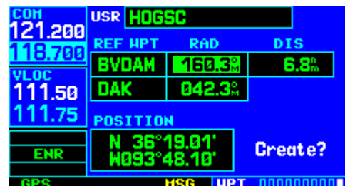
Figure 7-41 Radial Field Highlighted
